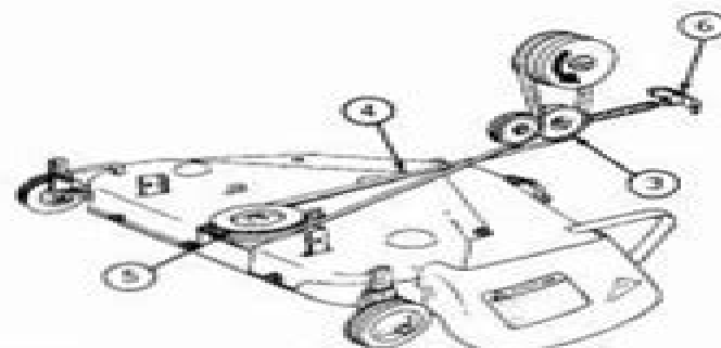
Fig. 5-Replacing Drive Belt
