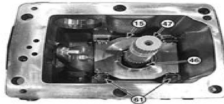
Servo Plate Installation
