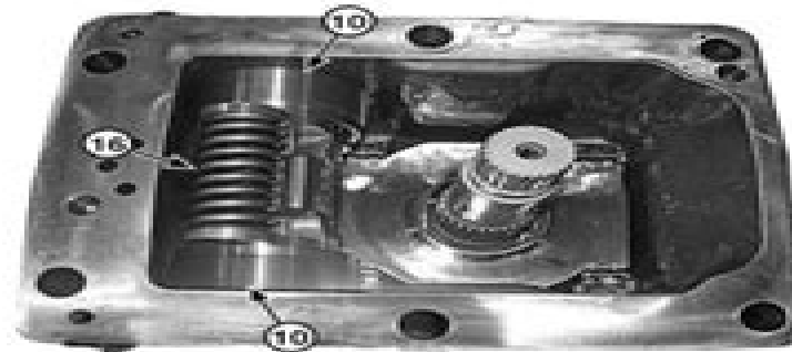
Servo Piston Installation
