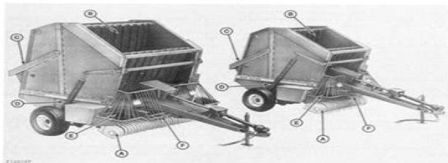
A—Pickup B—Upper Belt
