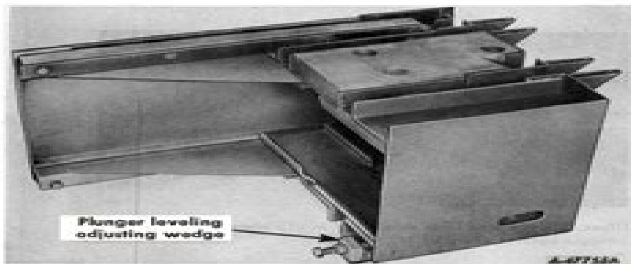
Illustr. 31A - This wedge is used to level plunger so plunger hay knife is parallel to the stationary knife.
