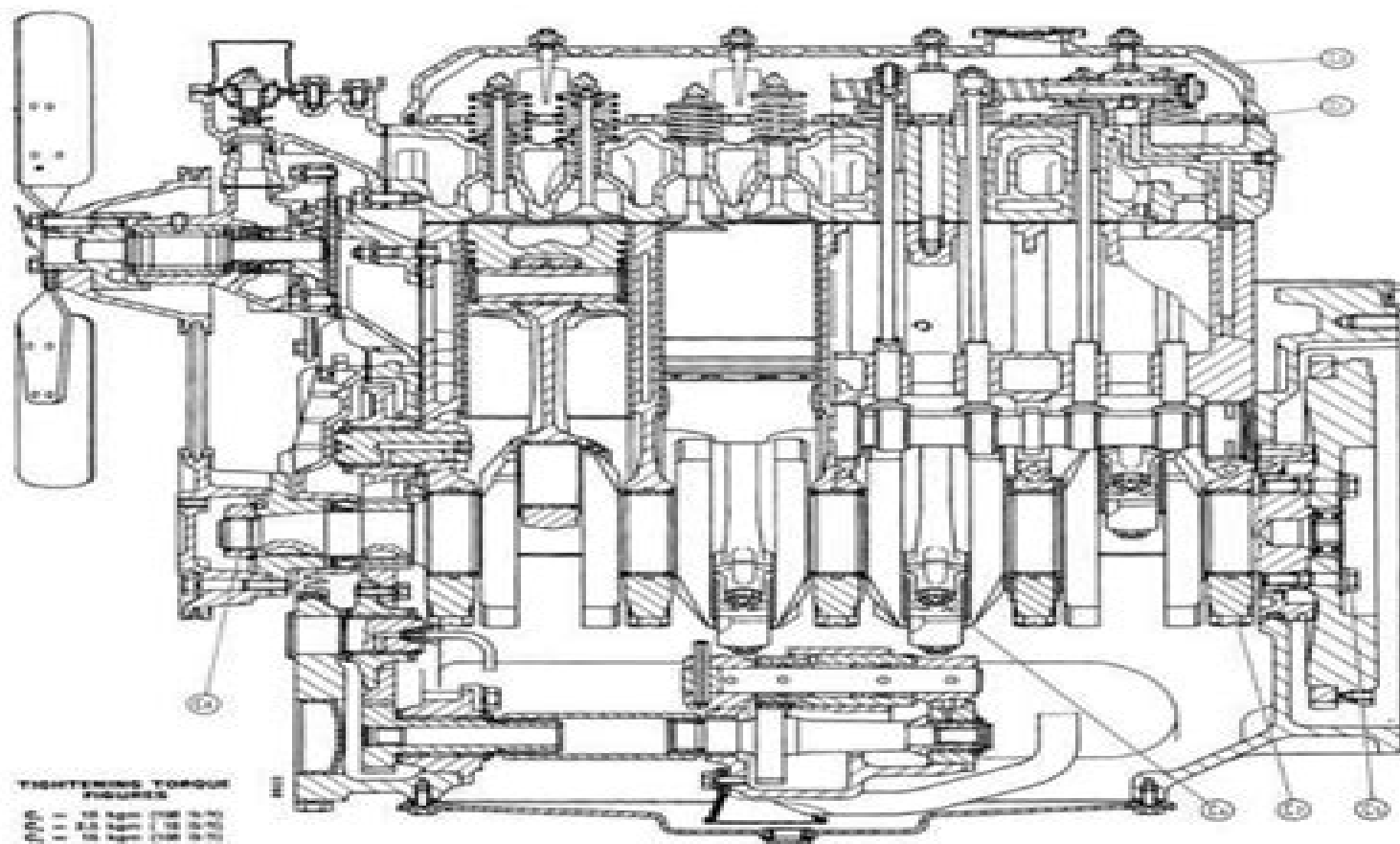
Longitudinal Section through 780 Engine
