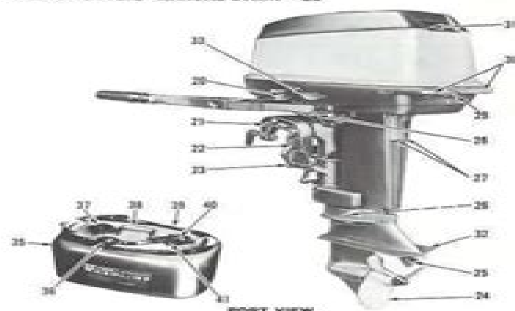
PORT VIEW
