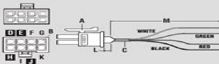
Figure 8 — Signal Wire Harness
