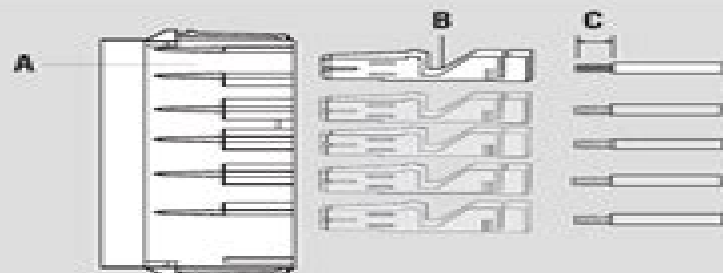
Figure 7 — Controller Molex Connector
