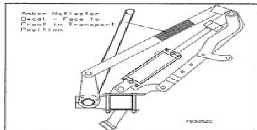
Figure 2.2c: Amber Decal Mount Locations
