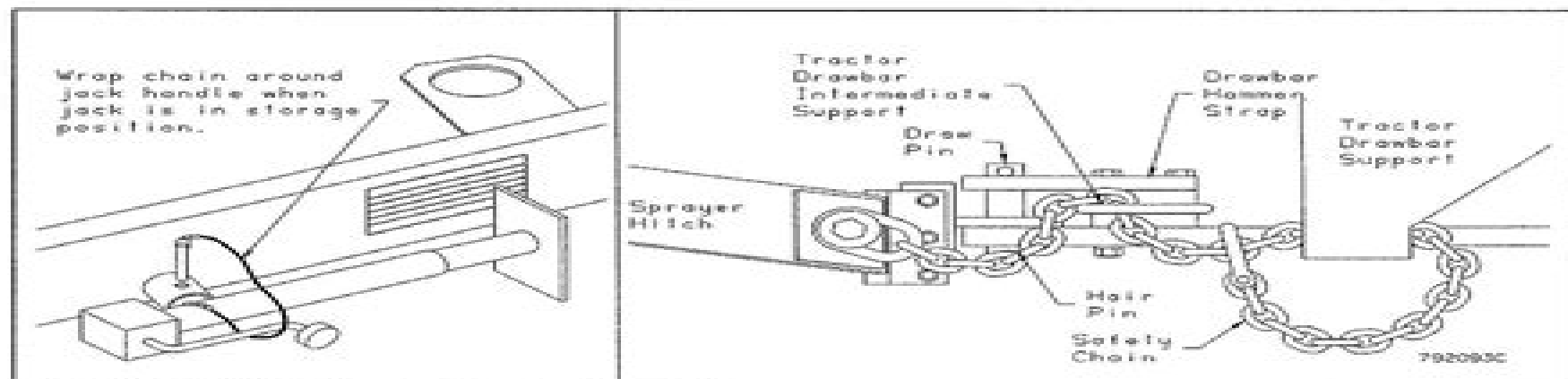
FIGURE 2.2d: Safety Chain and Tractor Connection
