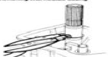
Fig. 7 Removing mainshaft stop
