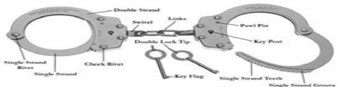
HANDCUFF NOMENCLATURE
