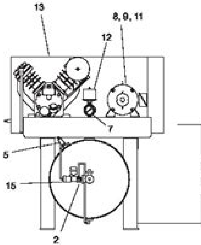
FIGURE 8. TYPICAL COUPLED RECEPTOR MOUNTED ELECTRIC PACKAGES.
