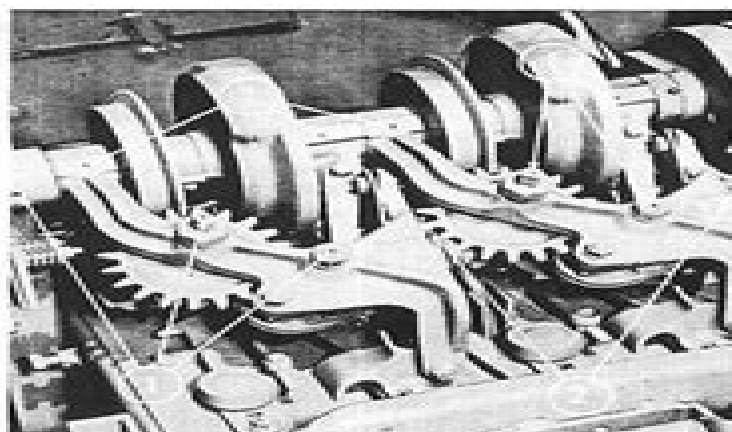
Fig. 5 Knottter Lubrication 1. \frac{1}{4} " Allen Head Plugs 2. \frac{1}{4} " Pipe Plugs
