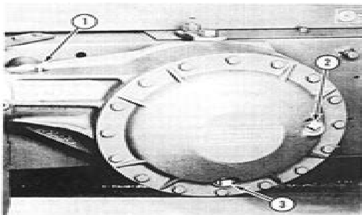
Fig. 3 Main Gear Housing 1. Breather 2. Filter plug opening 3. Drain plug
