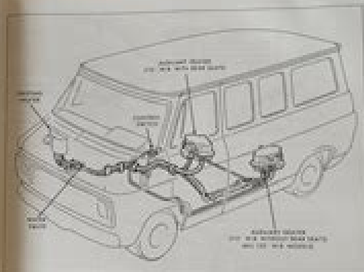
Fig. 10 Auxiliary Heater Installation
