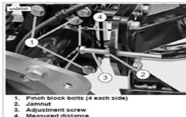
Figure 5-8. Adjust Axle
