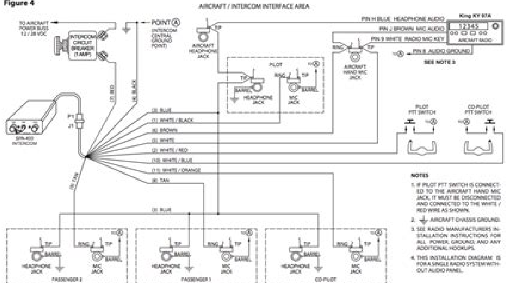
SPA-400 – King KY 97A Radio Installation Wiring Diagram
