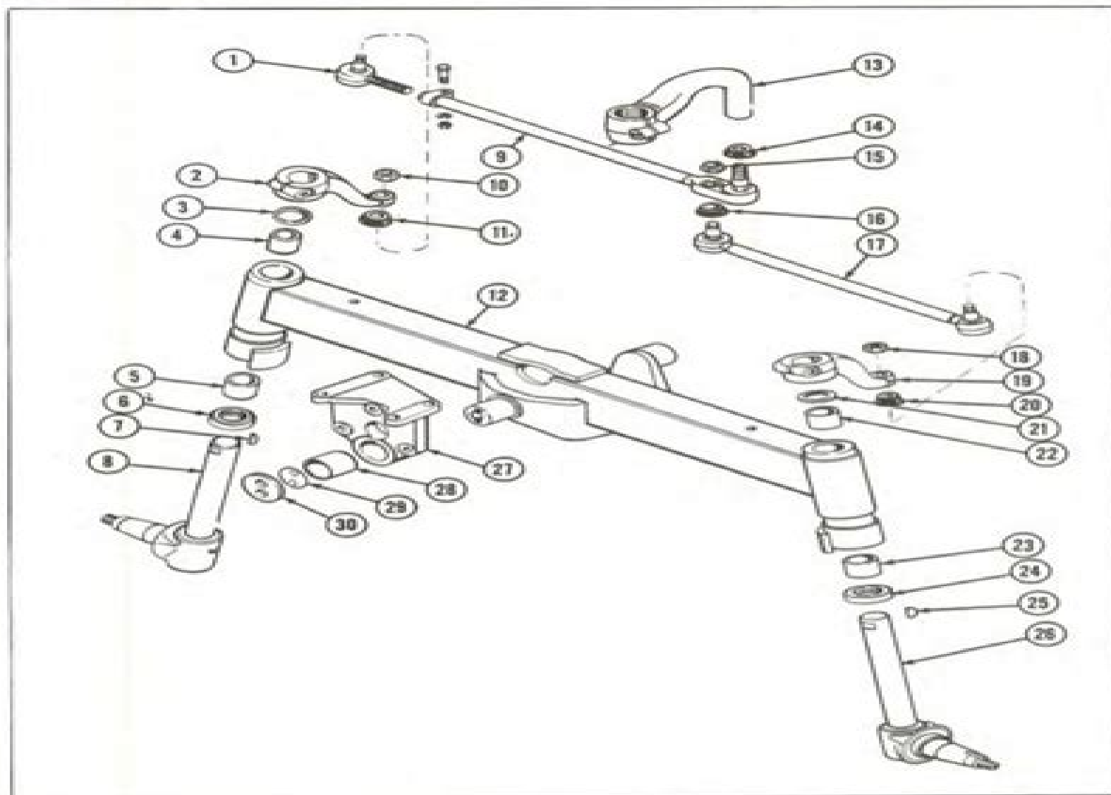
Fig. 3 - MF 65 Utility Front Axle Assembly Nomenclature.
