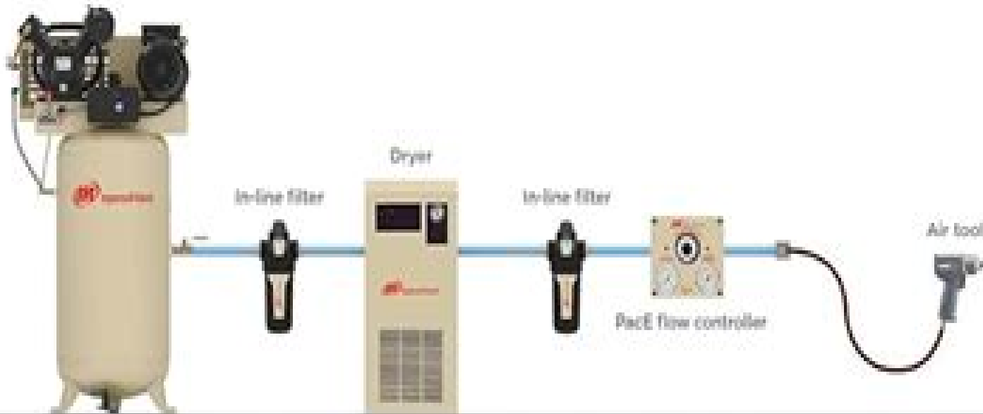
Reciprocating Air Compressor
