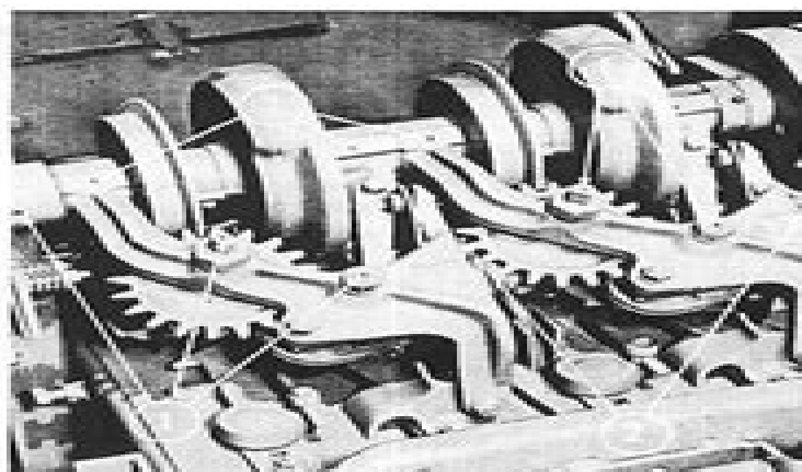
Fig. 5 Knotter Lubrication 1. \frac{1}{4} " Allen Head Plugs 2. \frac{1}{4} " Pipe Plugs
