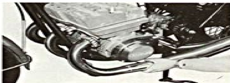
Fig. 7-1-23 Removing muffer
