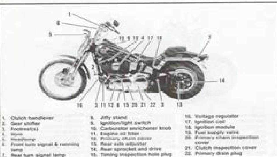
FIGURE 1-5. 1991 FXSTC - Left Side View
