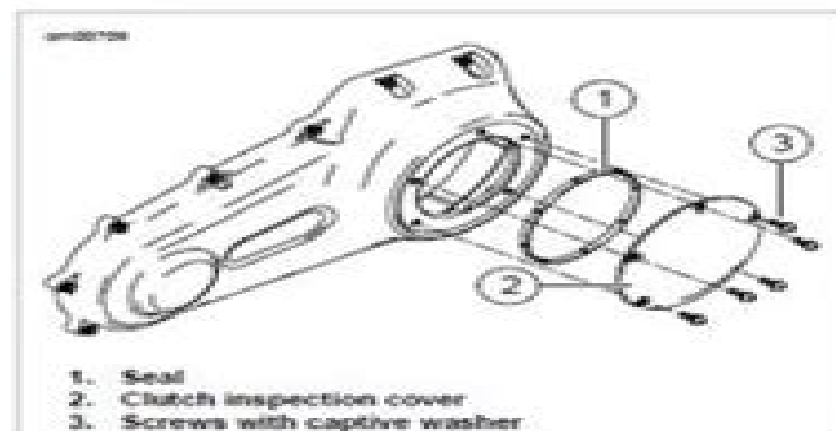
Figure 1-11. Clutch Cover
