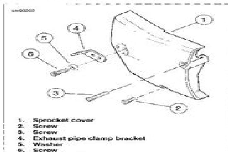
Figure 4-71. Sprocket Cover
