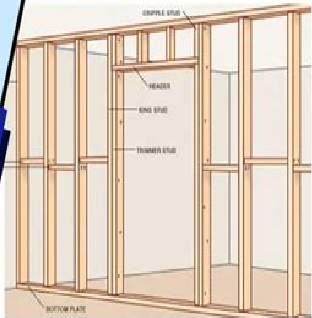
FRAMING OF AN INTERIOR WALL
