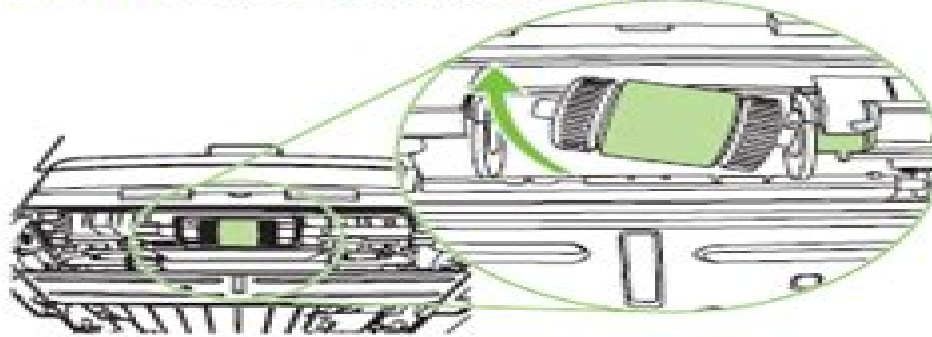
Figure 3-4 Replace the tray 2 pickup roller (4 of 7)
