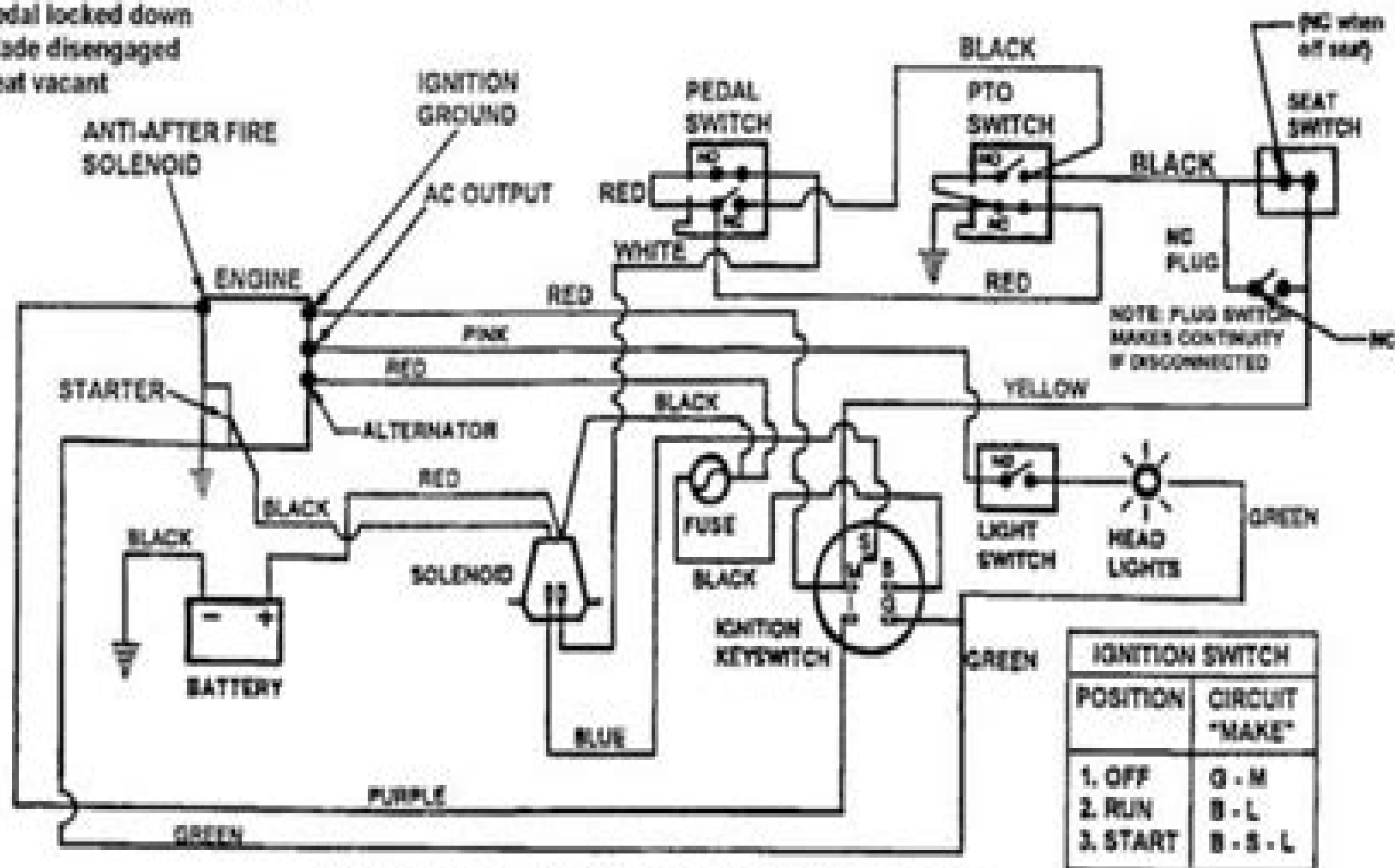
SCHEMATIC - WIRING HARNESS P.N. 2-6616 (MODELS: LT140H33DBV, LT140H33DB, LT145H38DBV & NLT145H38DBV)
