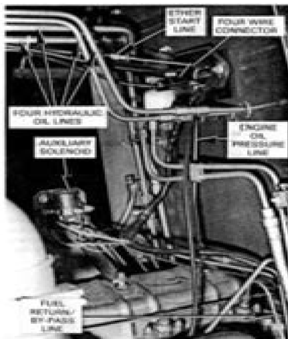
Fig. 3 — Identification of Parts — Viewing Left Side of Machine
