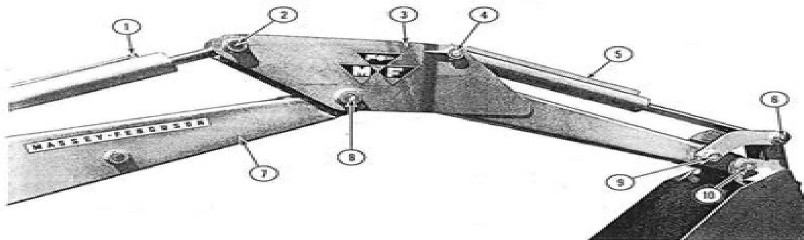
Fig. 8 - Dipperstick Assembly
