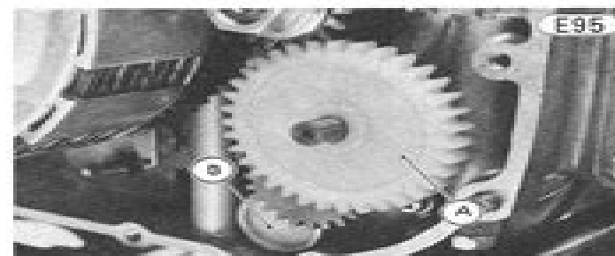
A. Oil Pump Drive Gear B. Oil Pump
