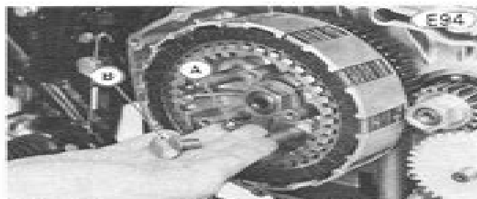
A. Steel Ball B. Spring Plate Pusher
