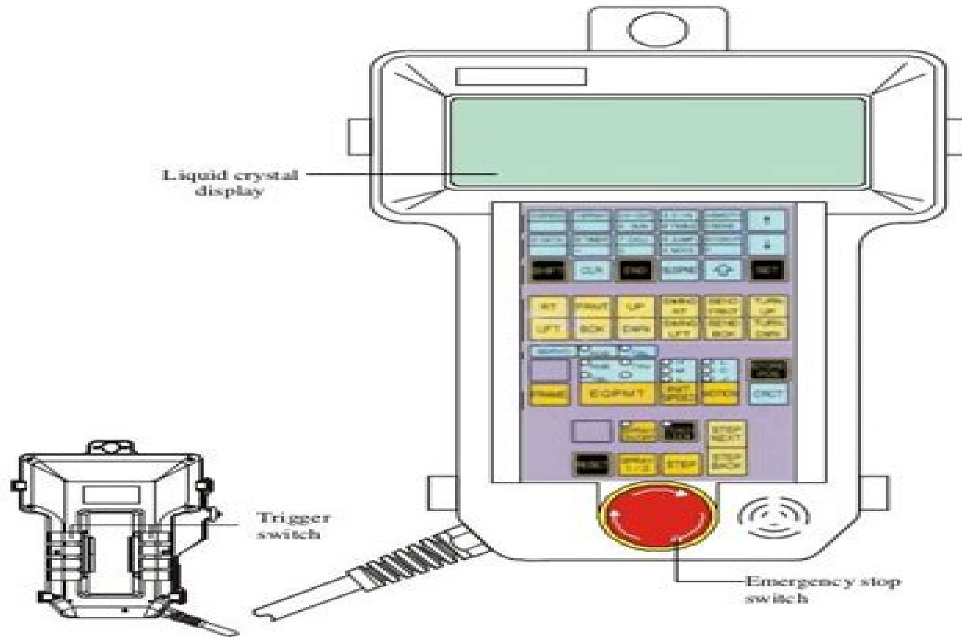
Back side of the explosion-proof teach pendant
