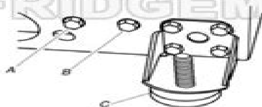
A. Rear roller adjustment screw B. Front roller adjustment screw C. Brake foot
