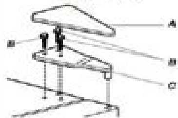
A. Top Hinge Cover B. 1/4" Hex-Head Hinge Screws C. Top Hinge
