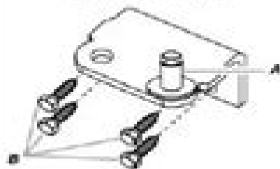
A. Hinge Pin B. 1/4" Hex-Head Hinge Screws
