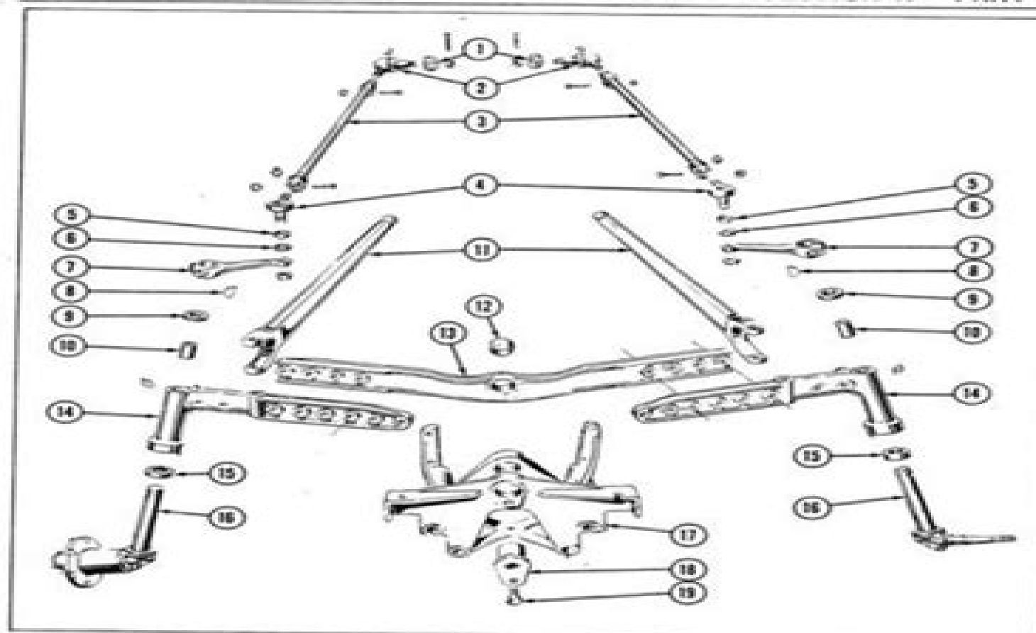
Fig. 1 - MF and TD 35 Front Axle Assembly Nomenclature
