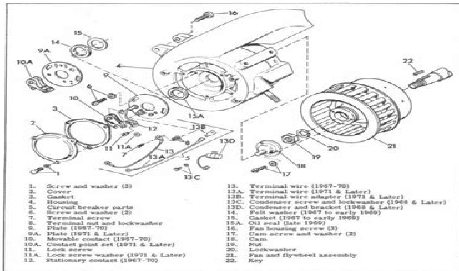
Figure 5F-12A. Circuit Breaker and Fan (1967 & Later D, 1969-1972 DC Models) - Exploded View
