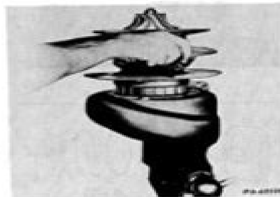
Illust. 6 Removing Core Assembly.
