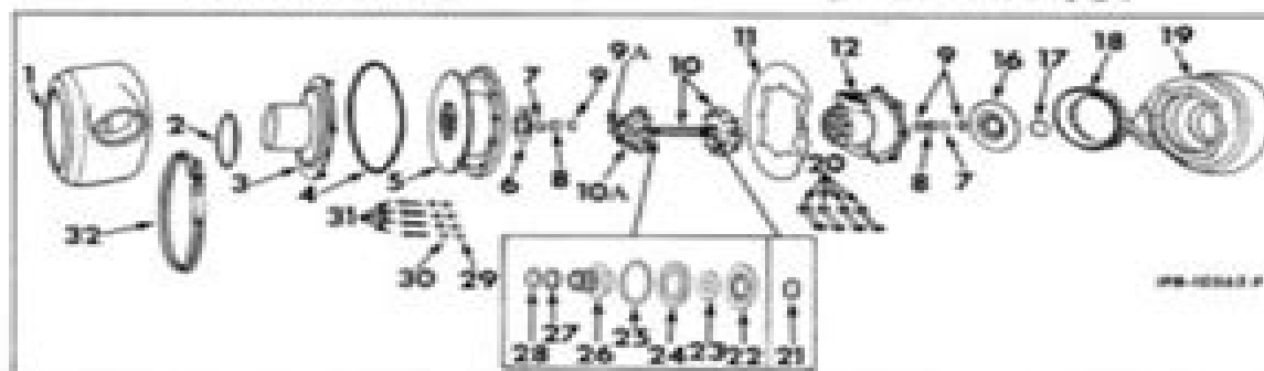
Illustr. 4 Exploded View of Turbocharger.
