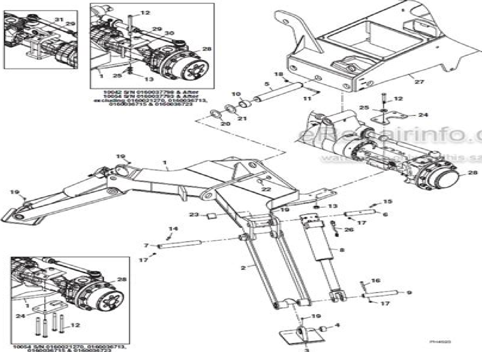
Figure 1-3 Outrigger Mounting
