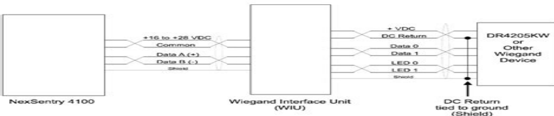
Figure 5: Typical Wiegand Connection
