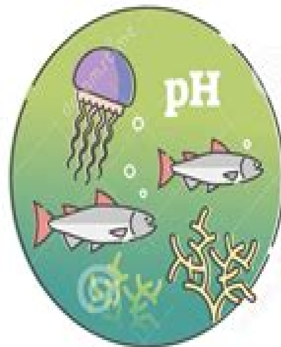
OCEAN ACIDIFICATION
