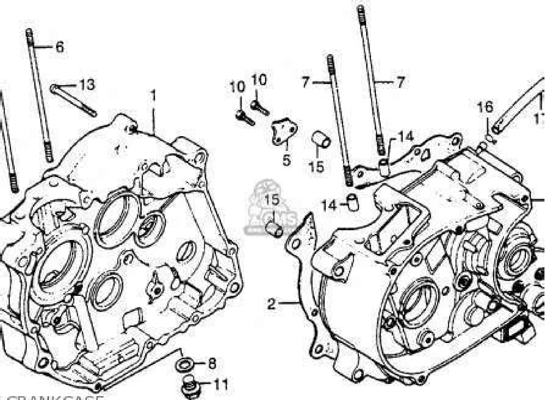
CRANKCASE
