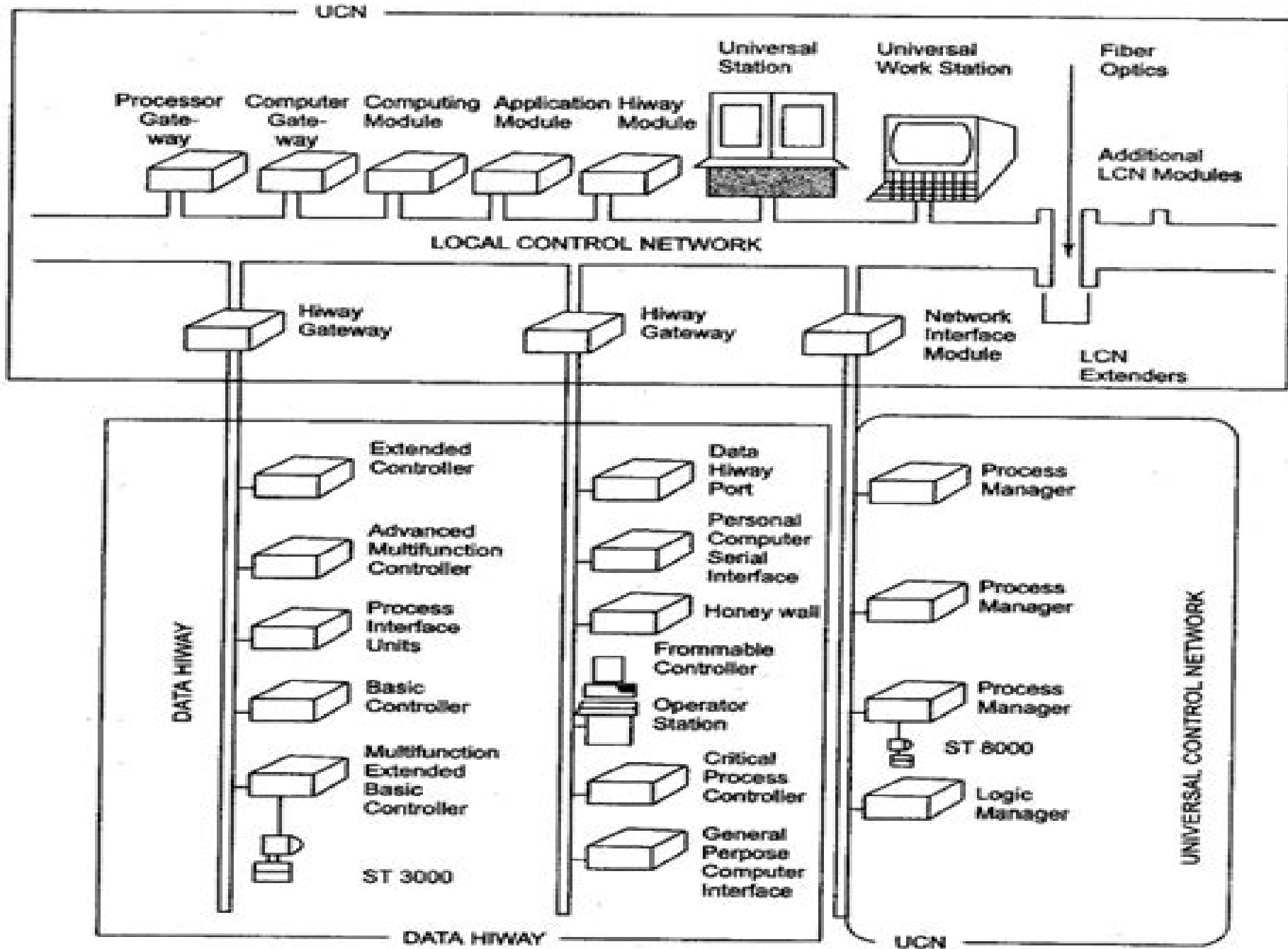
Fig. 21.77 TDC 3000 Architecture.
