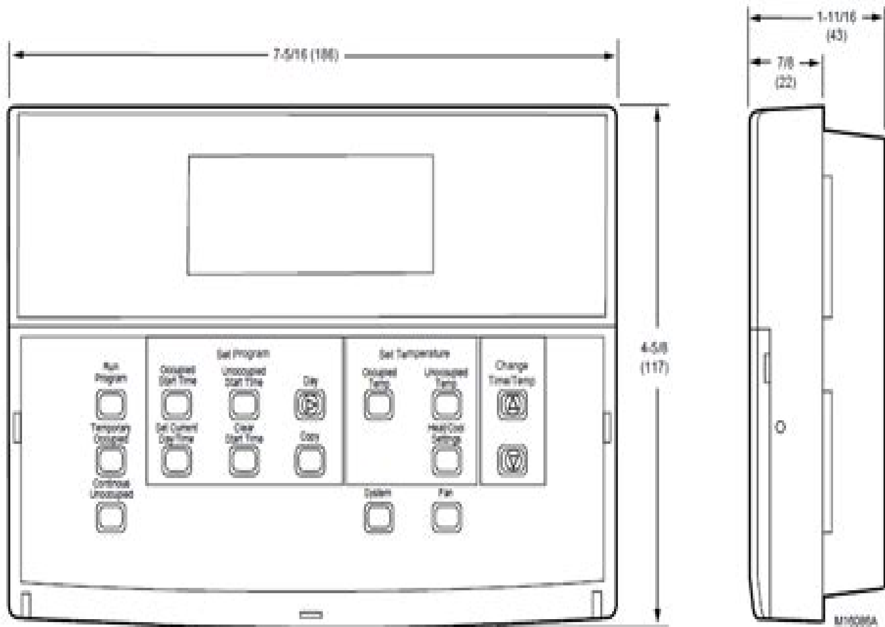
Fig. 3. T7300F/Q7300H dimensions in in. (mm).
