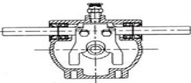
SECTION THROUGH ROCKER SHAFT AXIS
