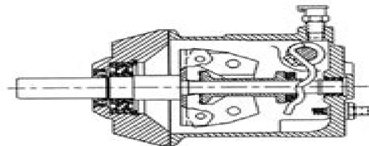
SECTION THROUGH MAIN SHAFT AXIS
