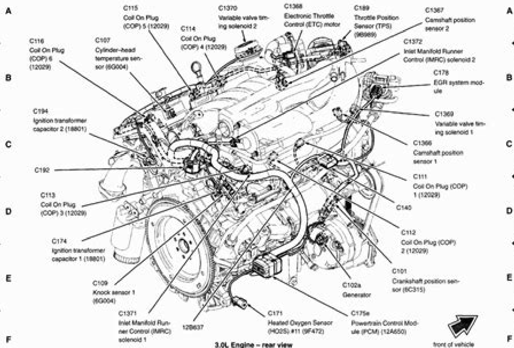
3.0L Engine - rear view
