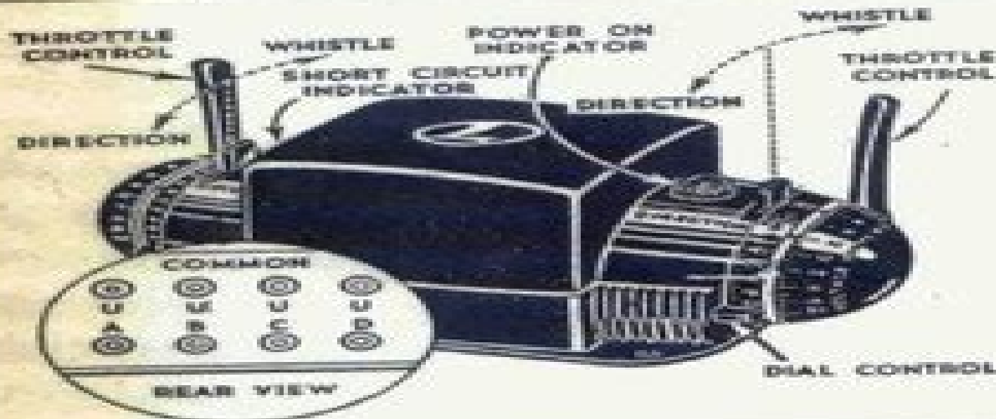
Figure 1—Type 2W "Mini-Control" Transformer.
