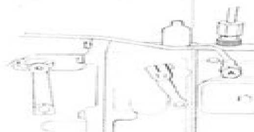
Fig. 12—On models equipped with C.A.V.-Minimec pump, loosen bleed screw "A" to bleed air from pump. Refer to text.
