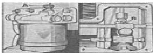
Fig. 11—On HR3 and HRW3 models, bleed screws are located at "A" on fuel filter body and "B" on fuel pump. Refer to text.
