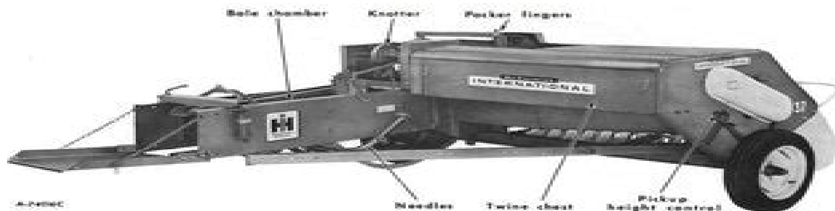
Illustr. 2A Right rear view of the 37 Twine Baler.
