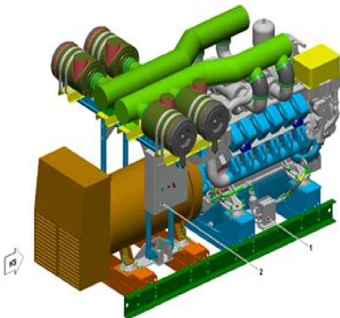
Figure 6: Engine-generator set with S4000 Gx3 engine – view on driving end
