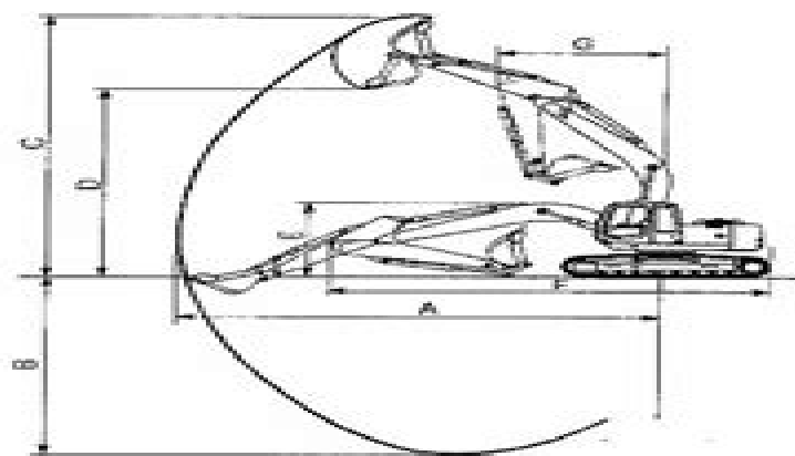
Face Shovel (Reversed hoe bucket)
