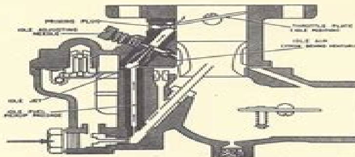
Fig. GR1—Zenith series 161-7 carburetor with only an idle mixture adjustment. In some installations a main power adjustment is provided by substituting a needle valve for the plug shown by a heavy arrow.
