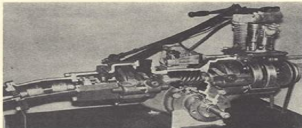
Fig. GR2—Cutaway of Gravely power plant showing Tee head engine having double internal flywheels, detachable main journals and crankpin and two-piece crankcase.
