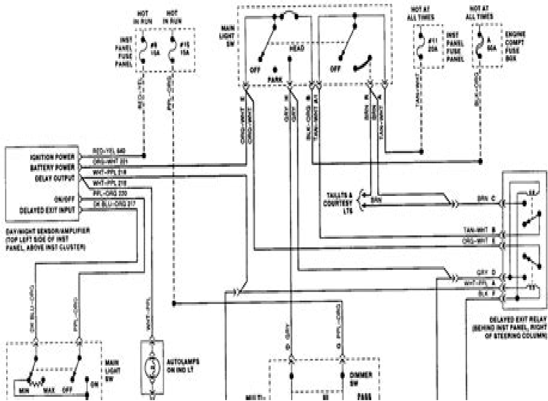
Fig. 4: Auto Headlight Dimmer Wiring Diagram Town Car (Automatic)
